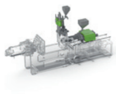
Injection unit in "V" position
