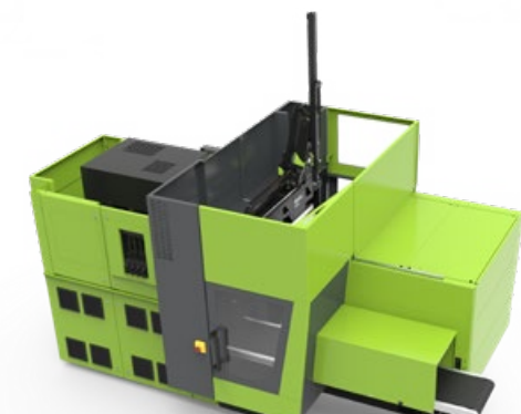
ENGEL e-motion 50 with expanded safety gate, integrated belt conveyor HLi and e-pic Z robots
